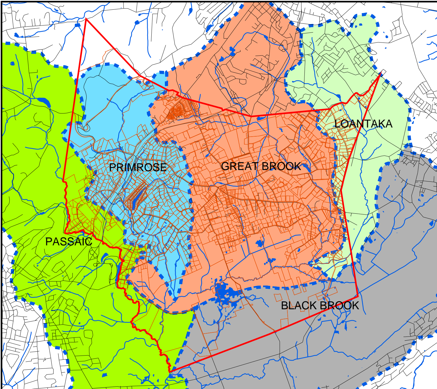
Figure 8 Drainage Basins
